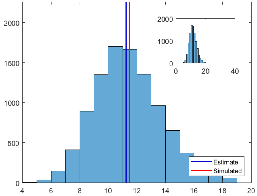
Figure B1. Simulated Value of Relationship Estimates Relaxing Independence of Inputs
